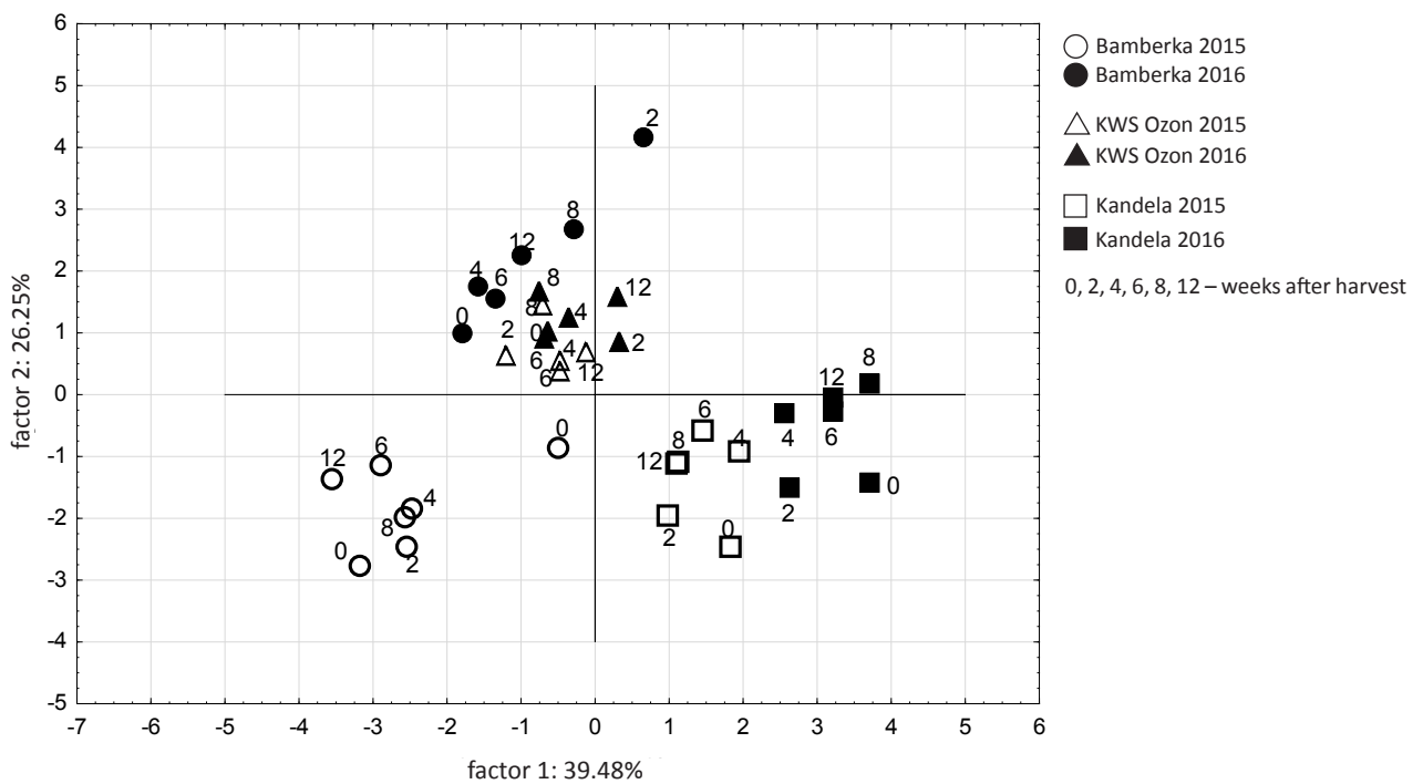
Figure 4. Loading plot of the first and second principal components of tested wheat cultivars on variables characterized the properties of starch-amylolytic complex of tested wheat cultivars.
