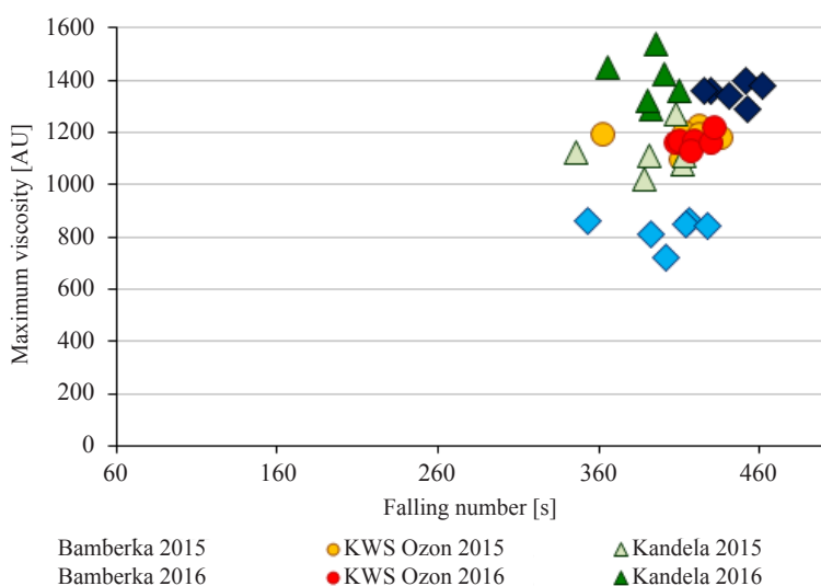
Figure 1. Falling number and maximum viscosity of flour of tested wheat cultivars from 2015 and 2016 harvest year.
